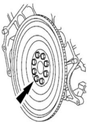
Fig. 278: Locating Flexplate Bolts Courtesy of FORD MOTOR CO.
